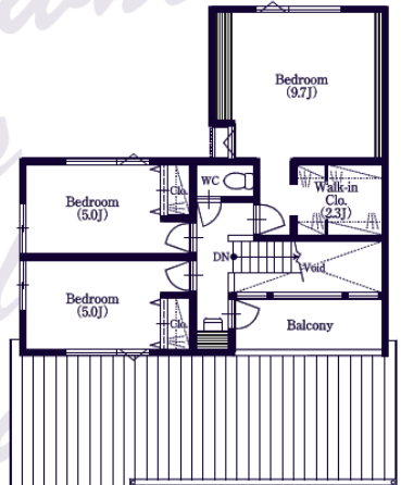
▶ The second floor plan view
